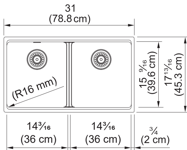
Dimensional Drawing
